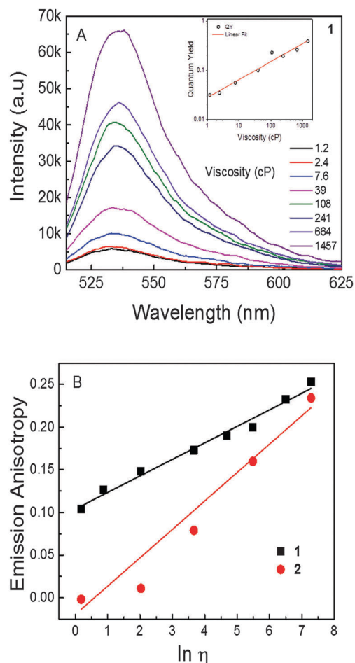
Fig. 2 (A) Emission spectra of dye 1 in different viscosity mixtures of ethanol: glycerol; inset: quantum yield as function of viscosity. (B) Steady state emission anisotropy of 1 and 2 as a function of viscosity.
